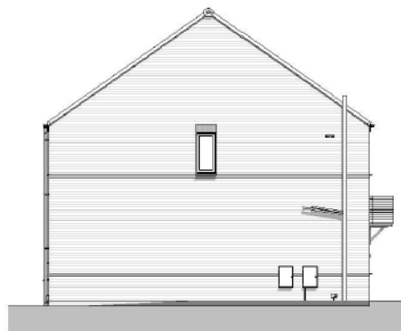
Left Elevation 1 : 100
